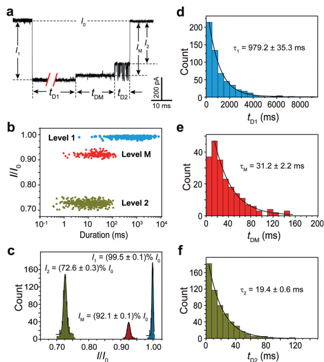
Figure 3. Statistical analysis of the signature events. a) A typical type-II signature event during the translocation of DNA1-FcCB[7] through \alpha HL under the identical conditions in Figure 2. I_0 stands for open pore current; I_{1,2} stands for the most probable current blockade of level 1-2; t_{D1-2} stands for the duration of the level 1-2. b) Scatter plots showing current blockades versus event durations of levels 1–2 in the signature events. The number of events is 500. c) Histograms of the current blockades of level 1-2. The solid lines are Gaussian fit to the histograms. d–f) Dwell time histograms of level 1-2. The solid lines are the single exponential fit to the histograms.
